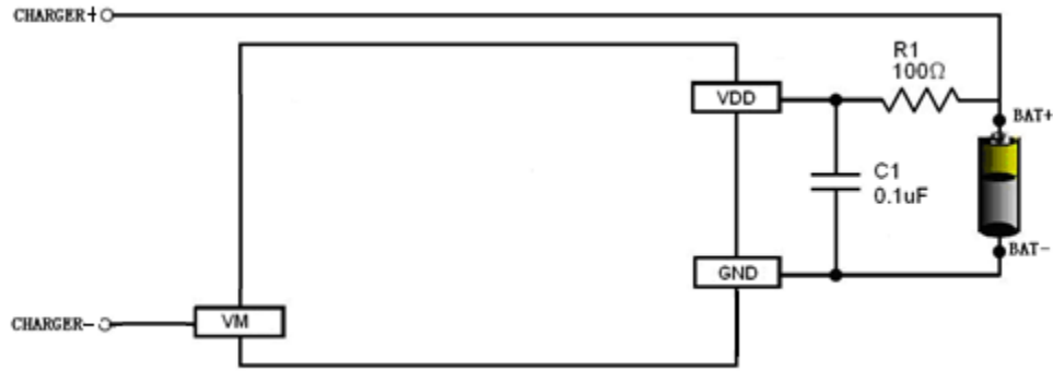
Fig 6 XR2104A in a Typical Battery Protection Circuit
